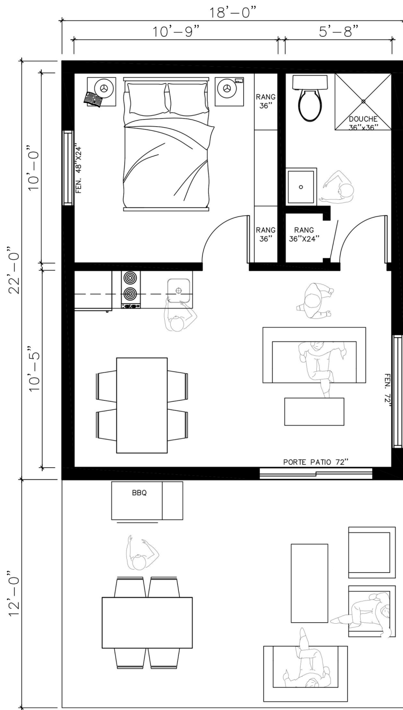
○ PLAN CABINE 18'-0" x 22'-0" ÉCHELLE: 1/4" = 1'-0"
